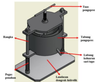
Figure 4. pressing machine parts
